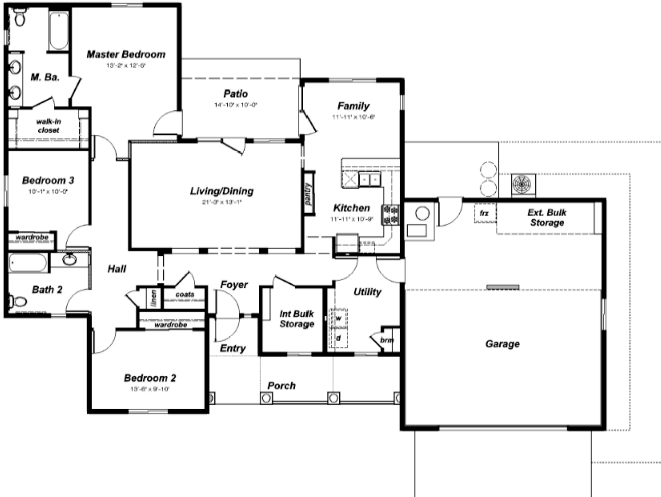
Kirtland AFB Unit F2 - Handicap Adaptable - 3BR (O4 - O5) Village II Provided 3 times (1,806 Gross S.F.)
